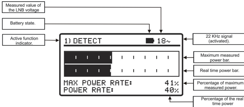
Figure 8.- DETECT function.
