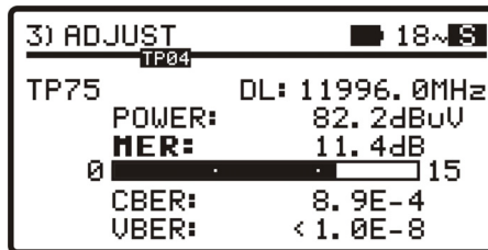
Figura 12.- DVB-S measurements with VBER.
