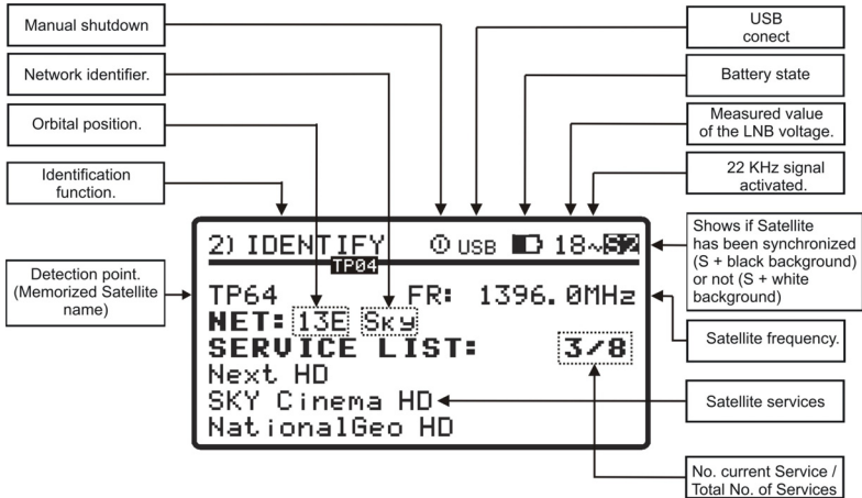
Figure 10.- Satellite identification screen.
