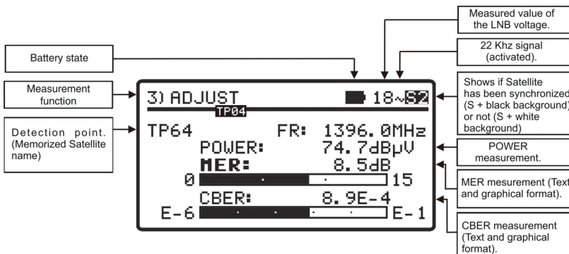
Figure 11.- Adjust function screen
