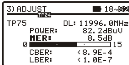
Figura 13.- DVB-S2 measurements with LBER.
